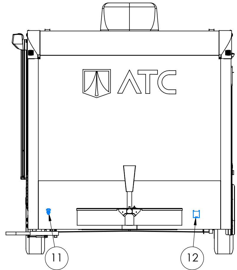
FRONT VIEW POPULAR OPTIONS FLOOR LAYOUT
